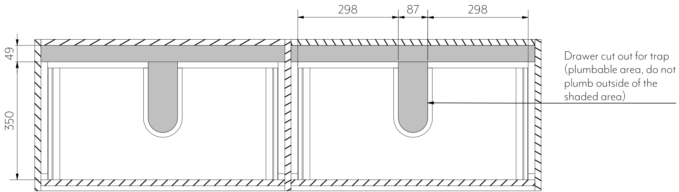
Section K-K
