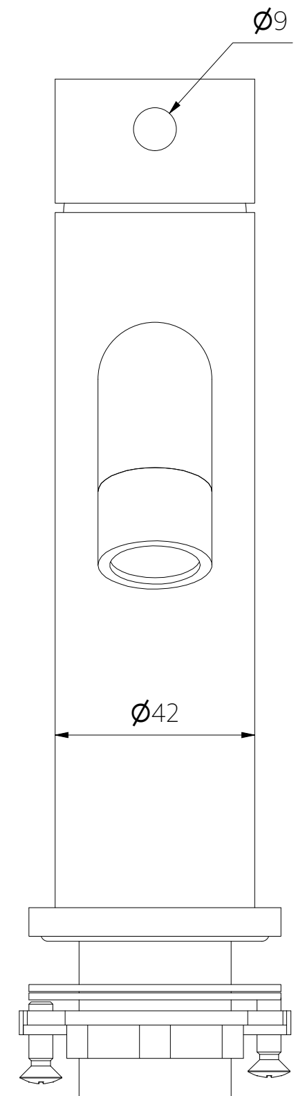
Front View
