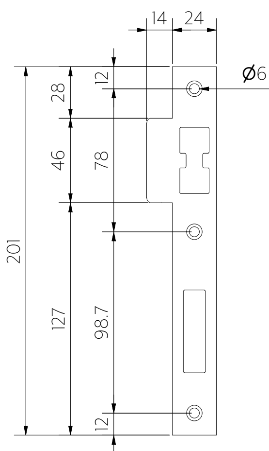
Front View (Right hand plate)
