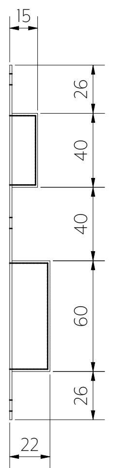
Side View (Dust Box)
