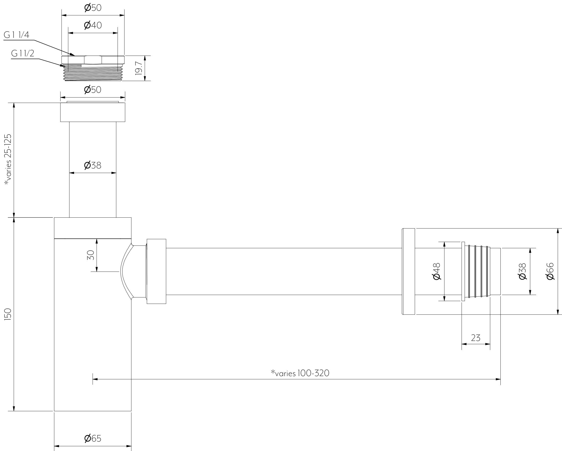
Front View
