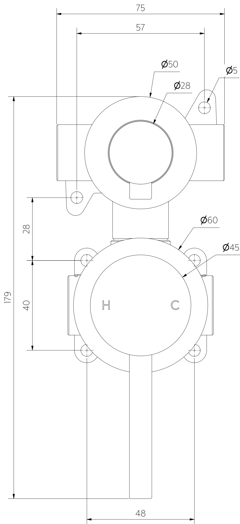
Front View
