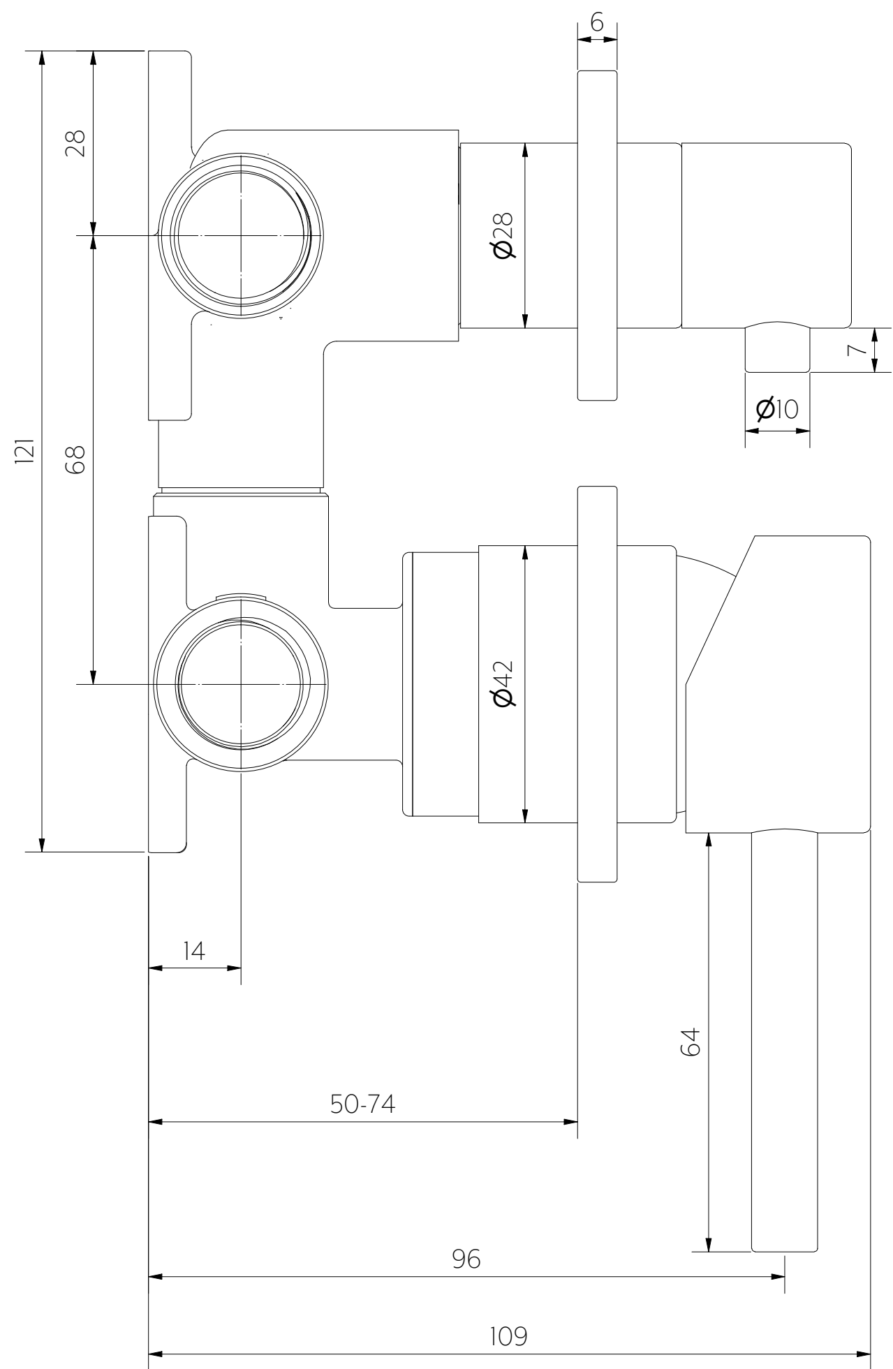
Side View
