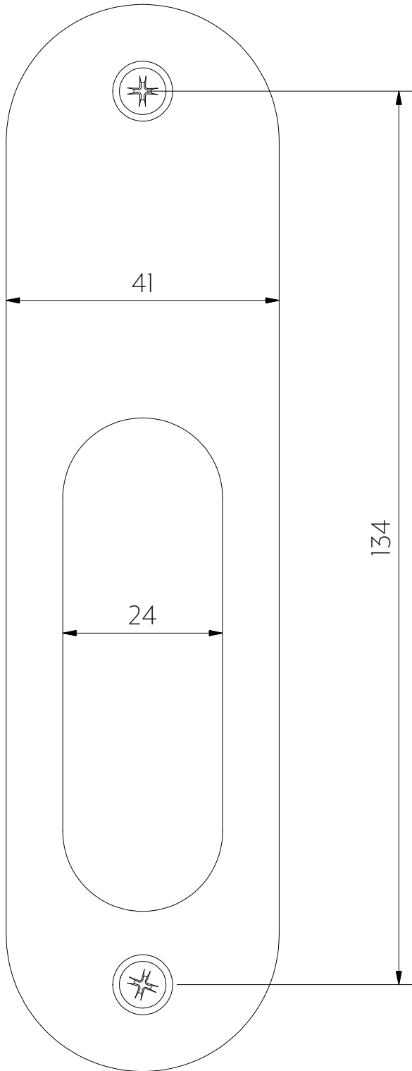
Back View
