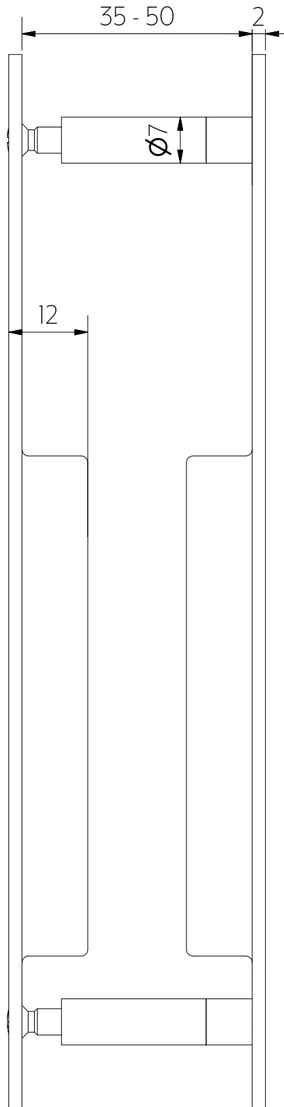
Side View
