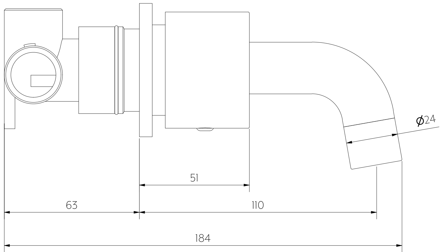
Side View
