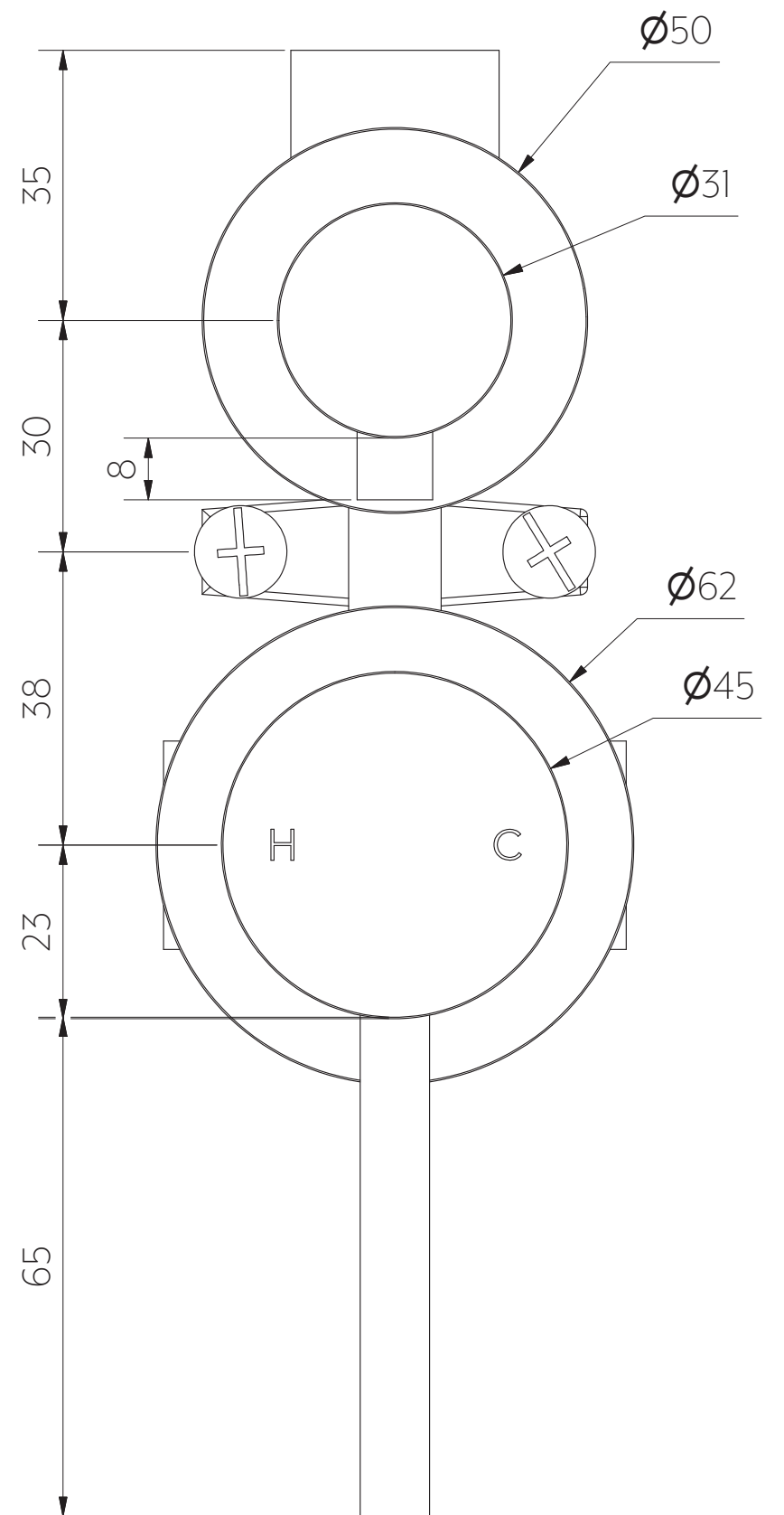
Front View
