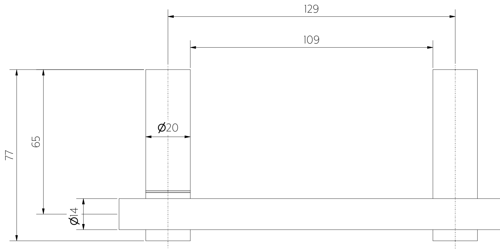
Top View
