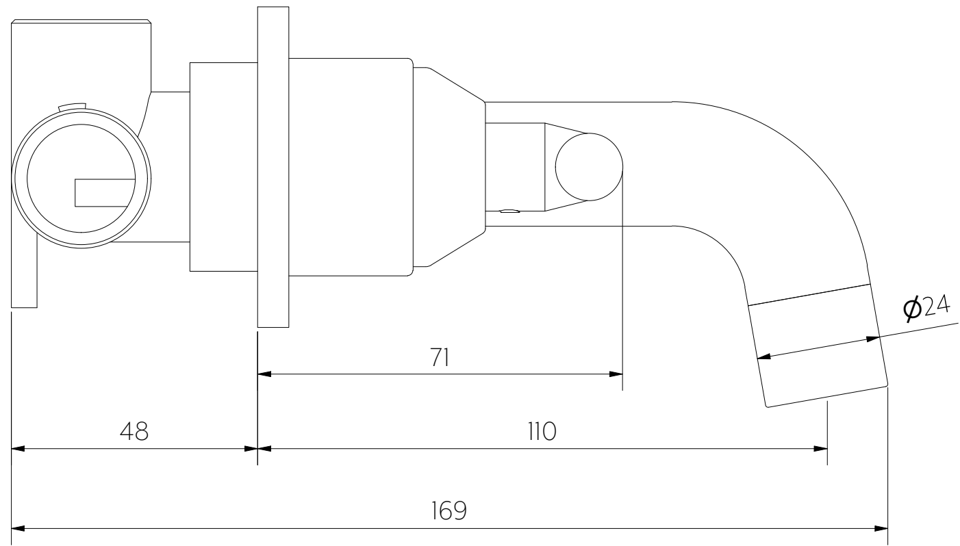
Side View
