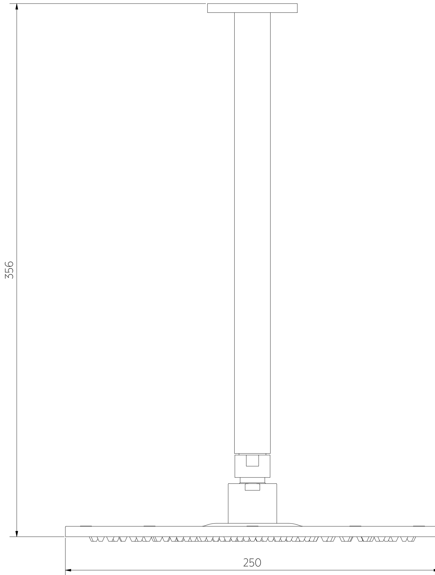
Front View
