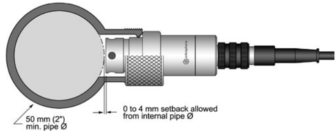
Weld-on Sensor Socket (29501)
