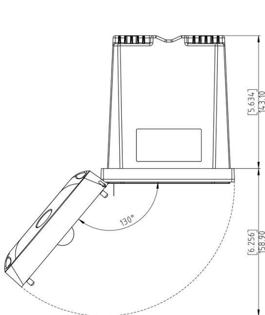
Door Opening Details
