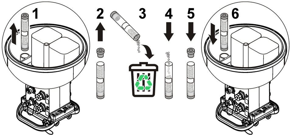
Figure 14 Desiccant replacement
