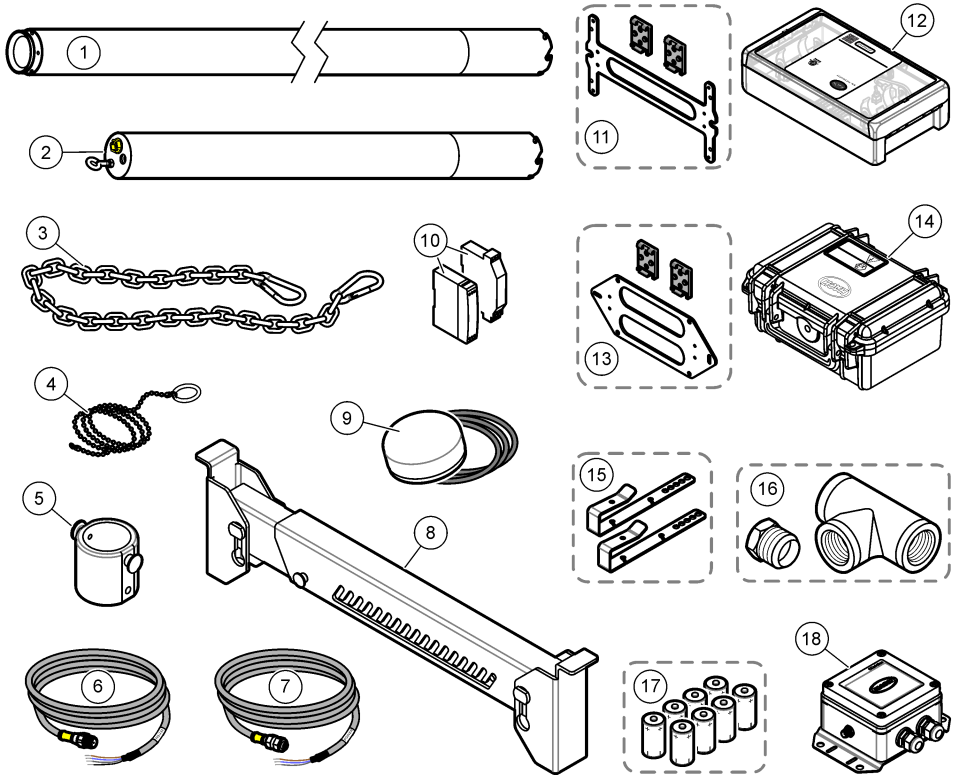
Figure 3 Accessories
