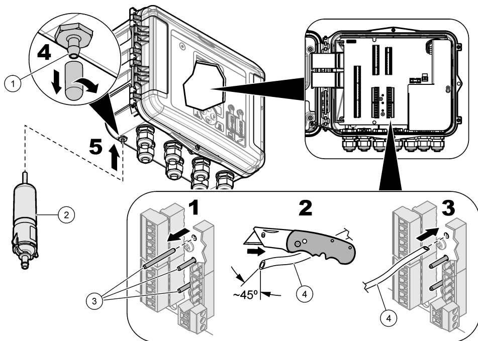
Figure 9 Air reference tube and desiccant installation
