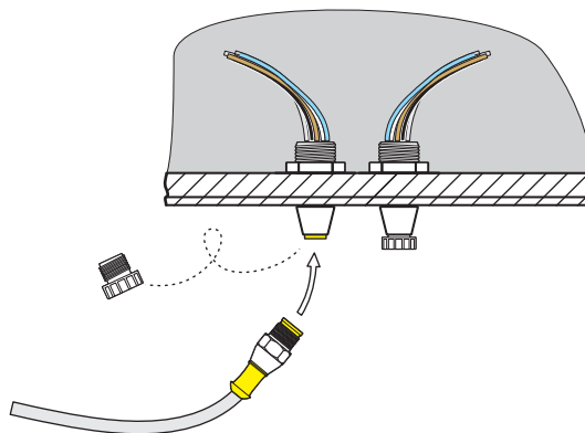
Figure 4 Connect sensor with quick connection
