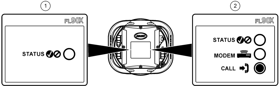
1 Instrument without modem 2 Instrument with modem
