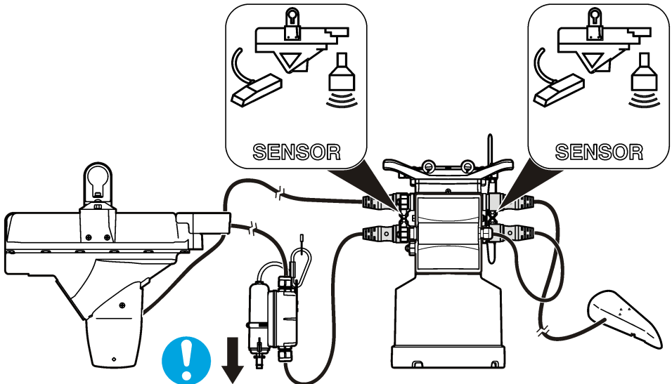
Figure 6 Attach a sensor to the logger
