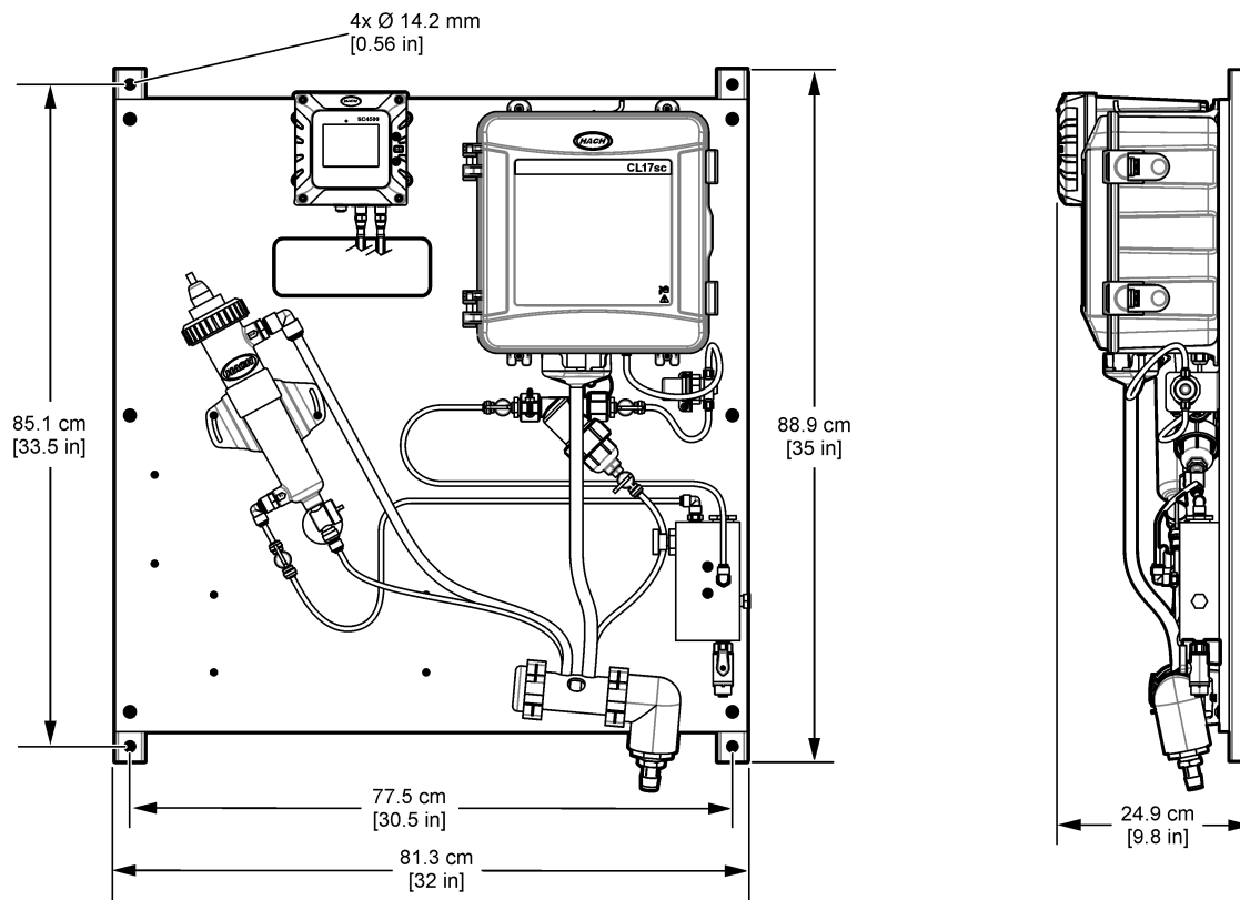
Figure 32 Product dimensions
