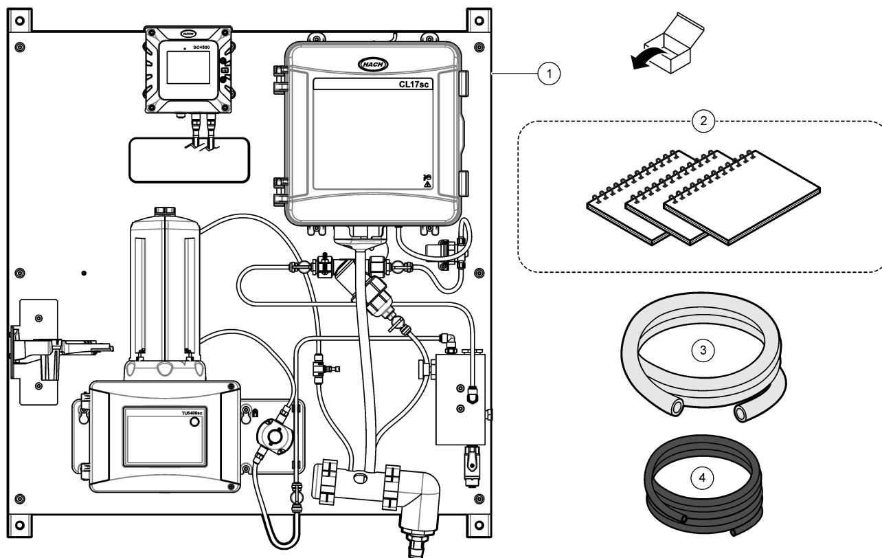
Figure 38 Product components
