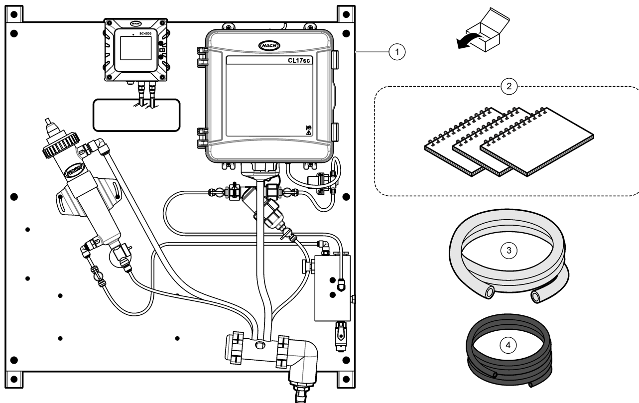
Figure 31 Product components
