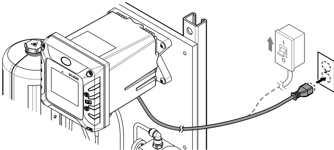
Figure 29 Apply power
