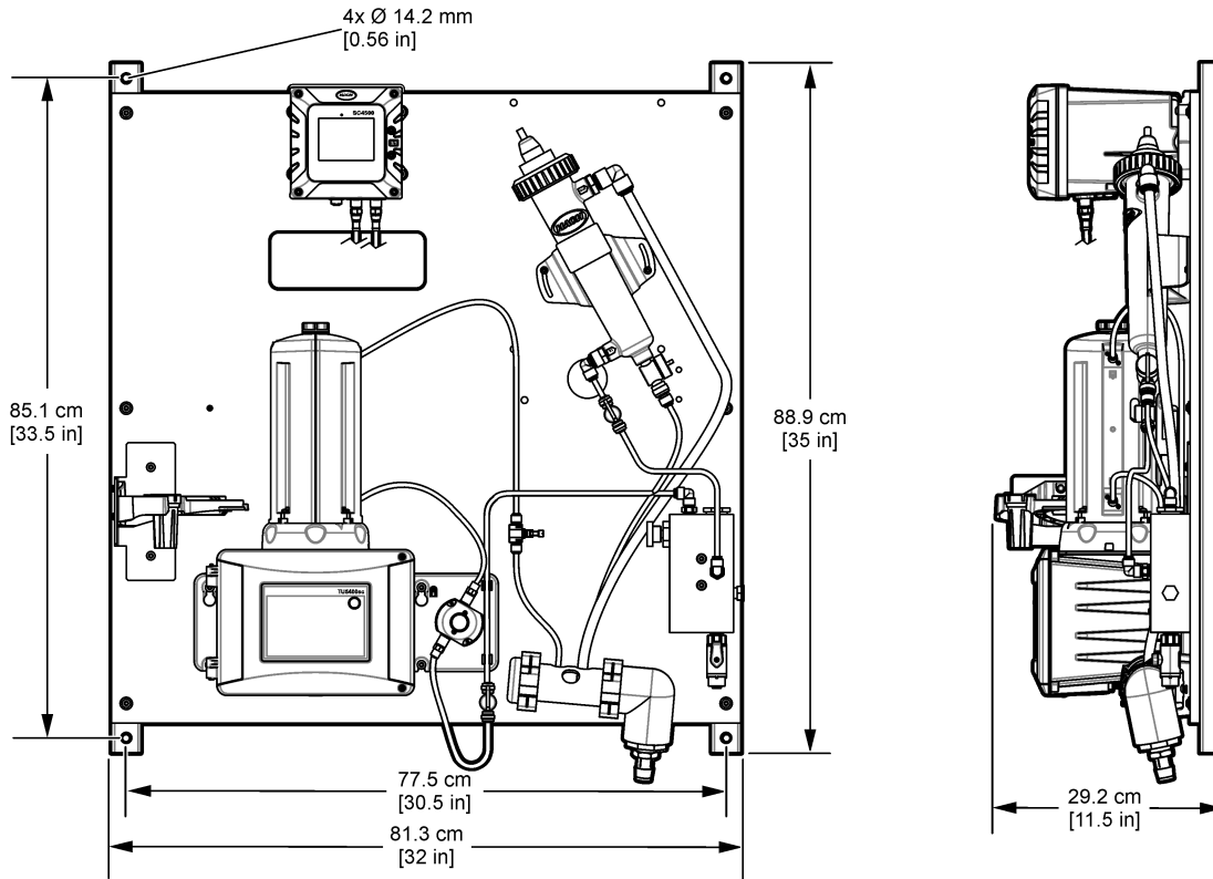
Figure 48 Hang the panel on a wall
