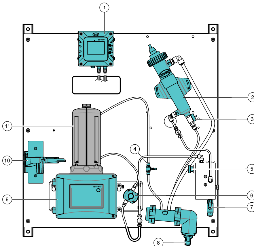
Figure 44 DPMP-TUPHD overview
