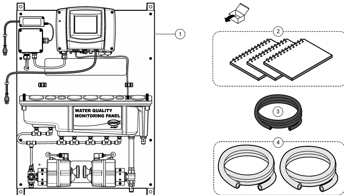
Figure 11 Product components
