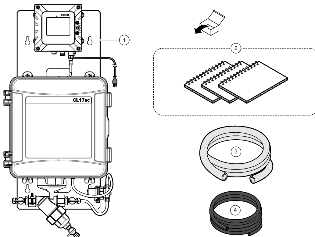
Figure 18 Product components
