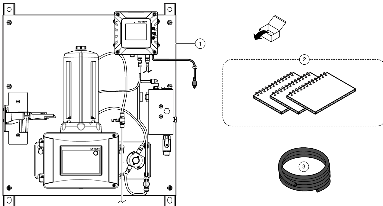
Figure 24 Product components
