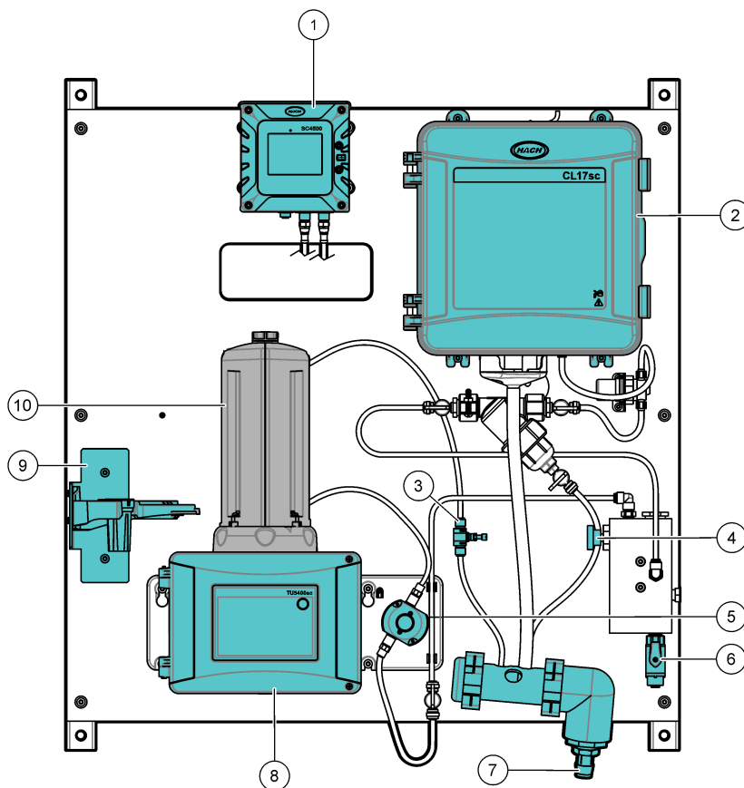
Figure 37 DPMP-CLTU overview
