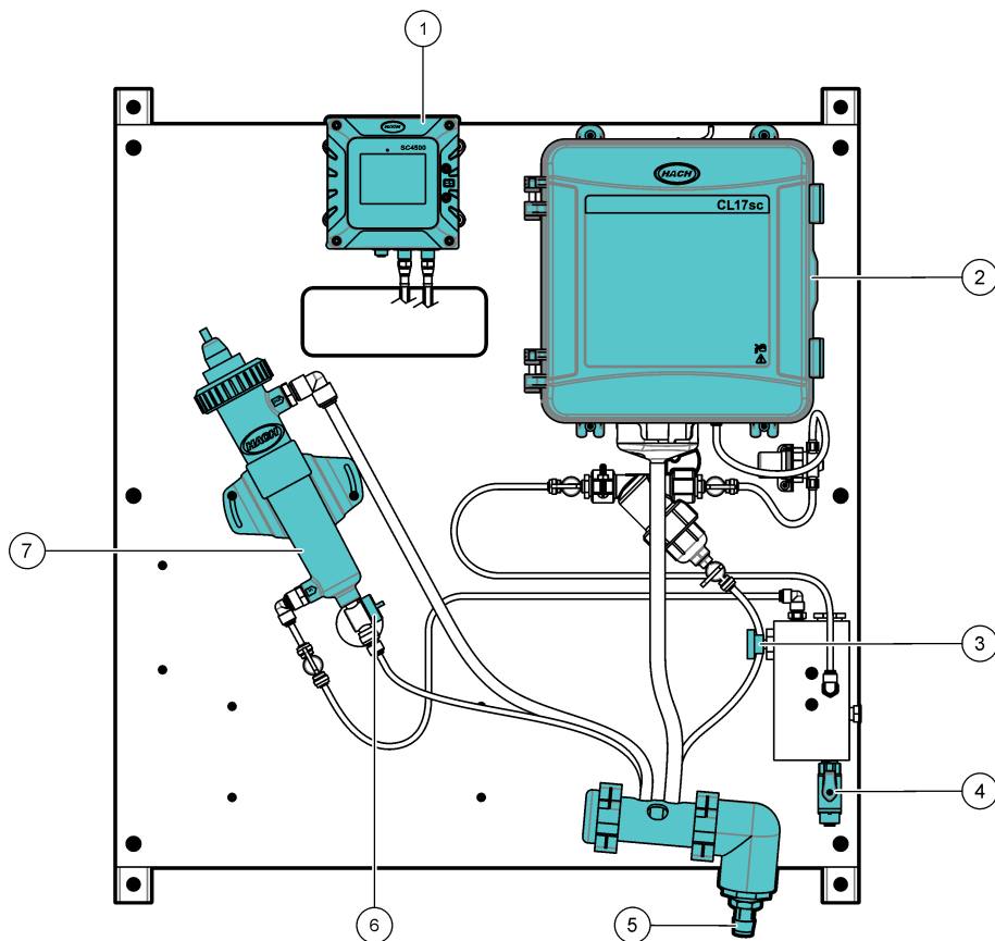
Figure 30 DPMP-CLPHD overview
