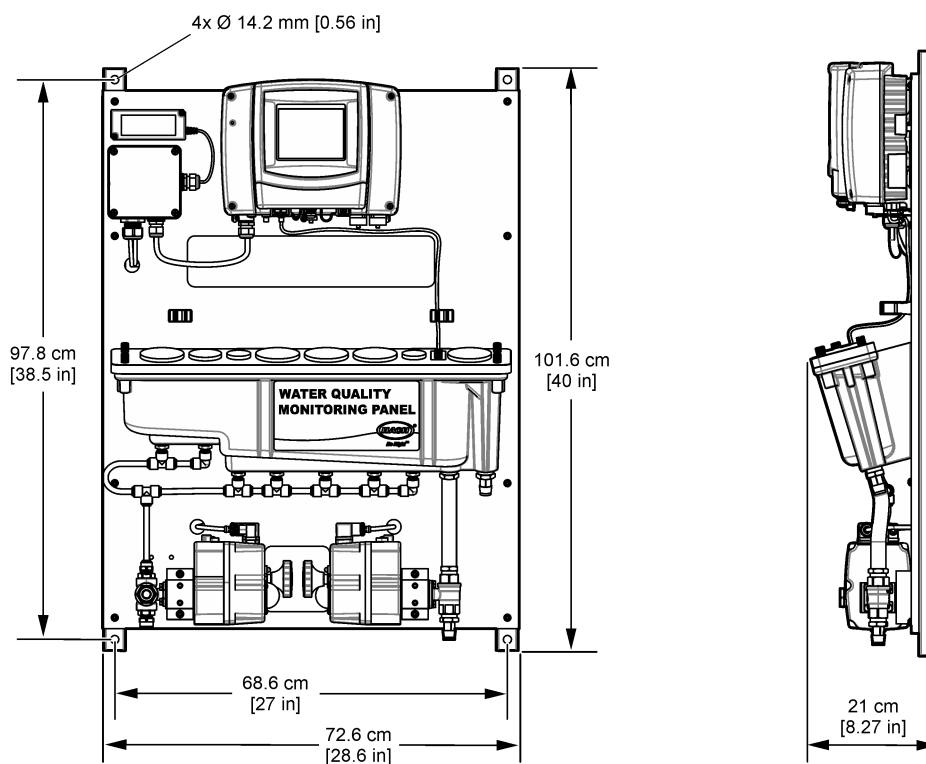
Figure 12 Product dimensions
