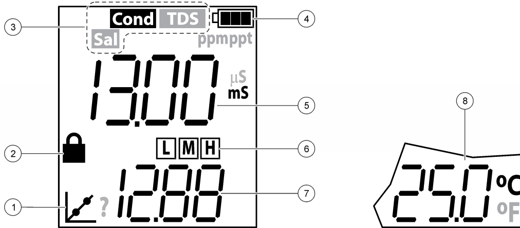
Figure 4 Display overview
