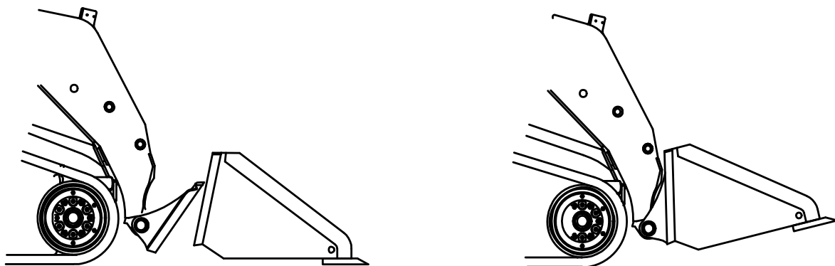
Figure 3.2a Quick Attach Mechanism Locked to Attachment
