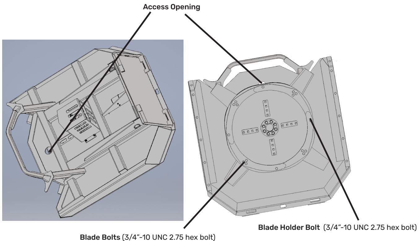
Figure 4.6a Blade Holder Access Opening & Bolt Diagram
