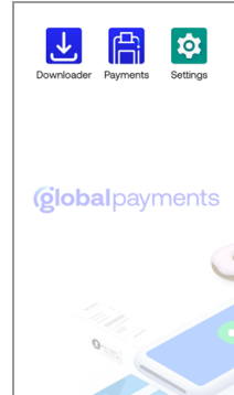
Launcher screen
