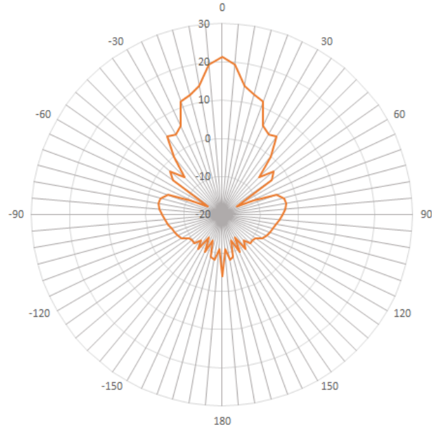
Directivity E plane @ 80GHz
