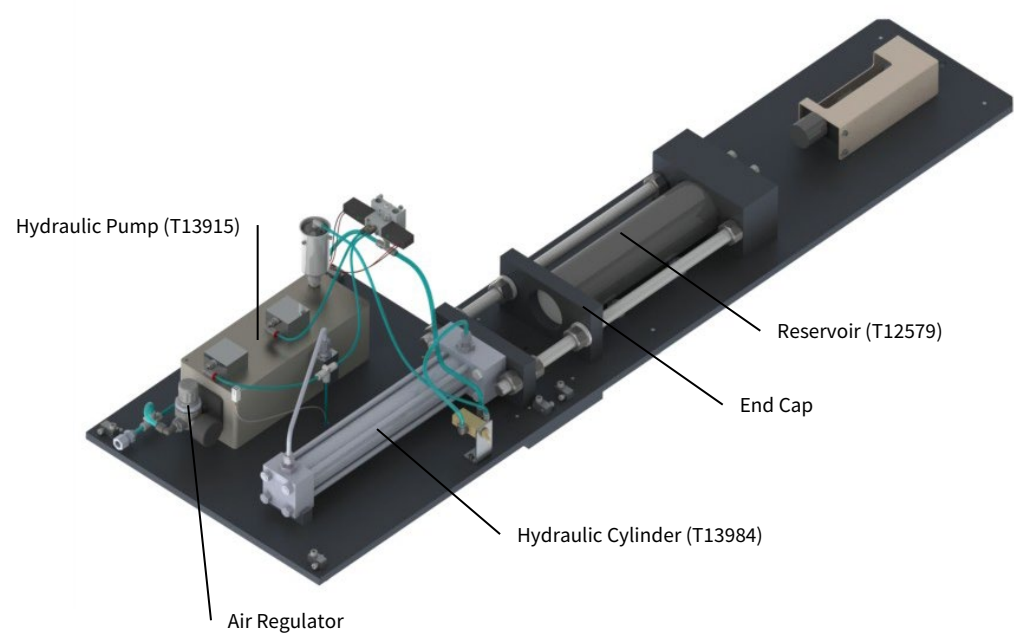
Figure 4. Main Interior Components
