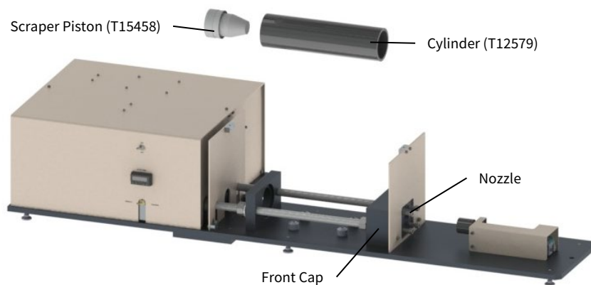
Figure 9. Wetted Parts
