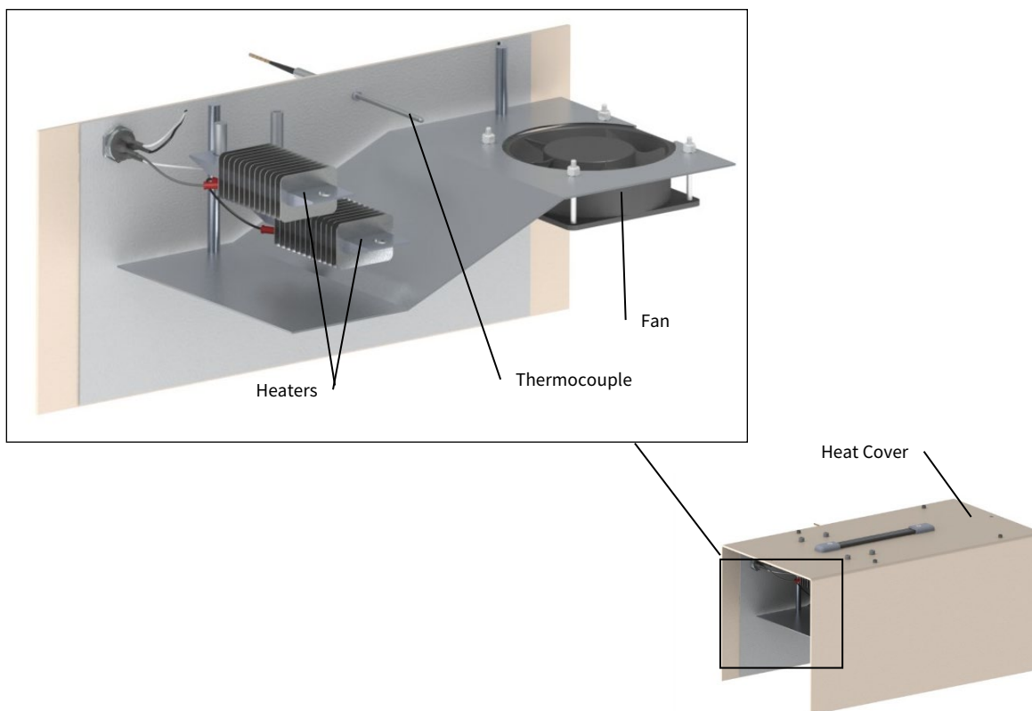
Figure 5. Heat Cover
