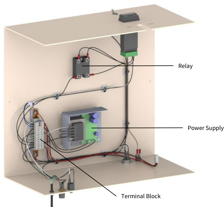
Figure 3. Electrical Cover
