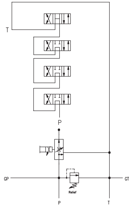
HYDRAULIC SCHEMATIC
