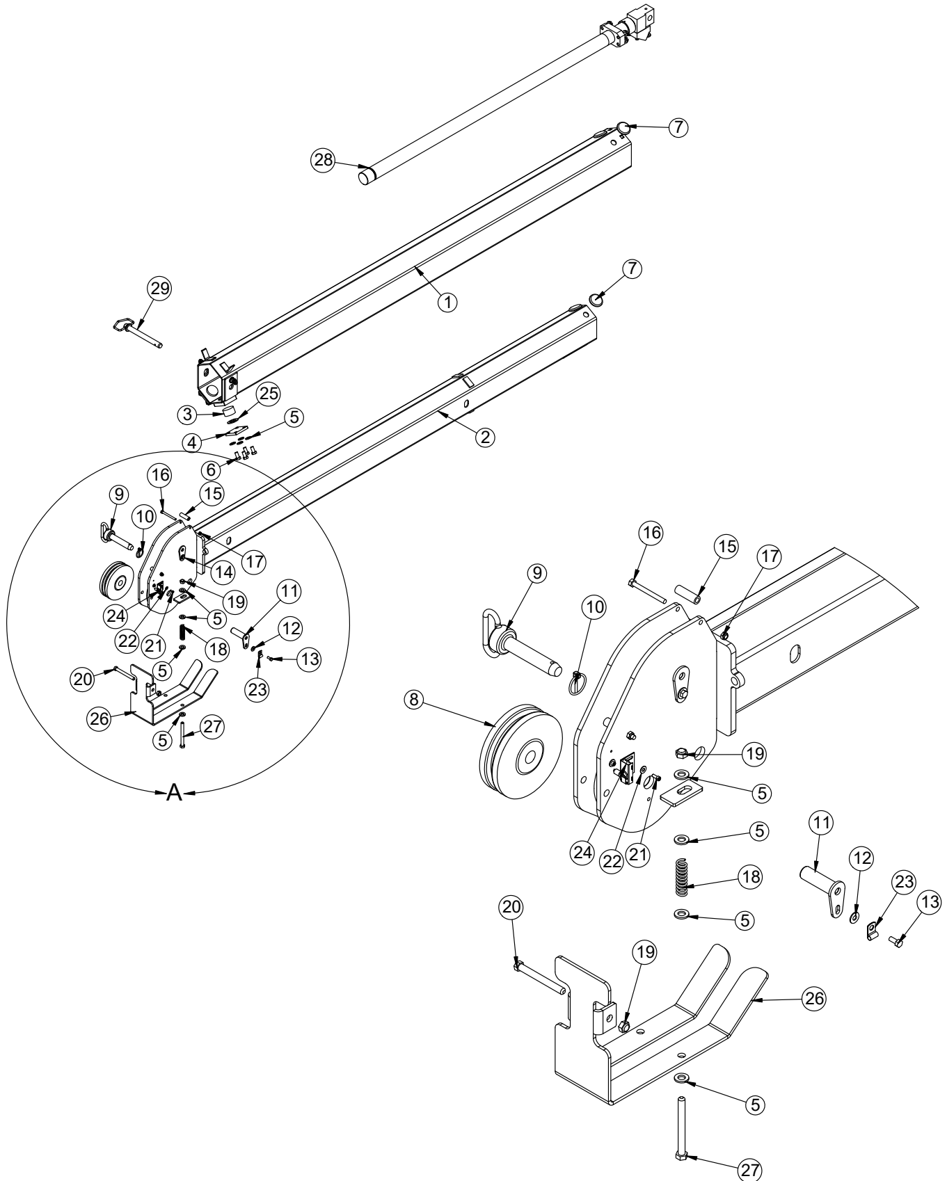
DETAIL A SCALE 1 : 9
