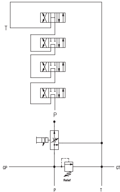
HYDRAULIC SCHEMATIC
